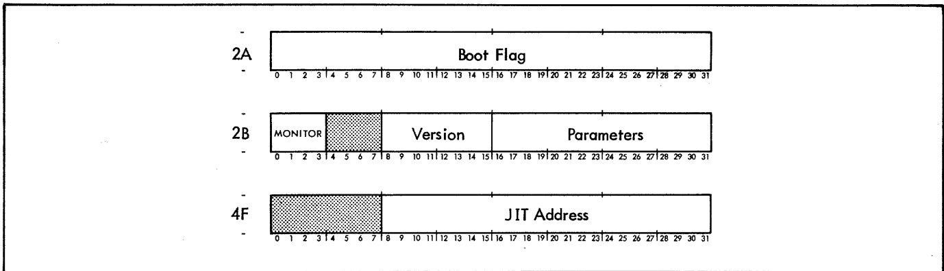
Figure 12. Locations Common to All Monitors
