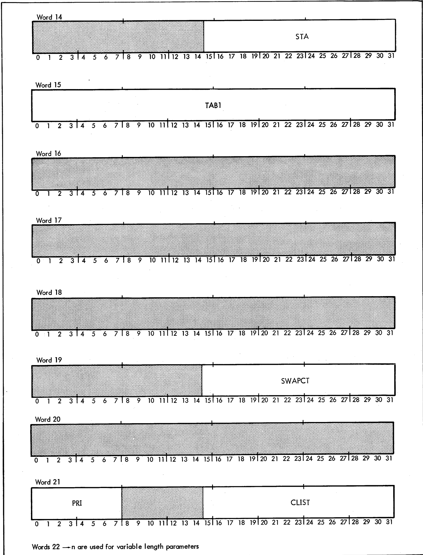
Figure 16. Format of the DDCB (cont.)
