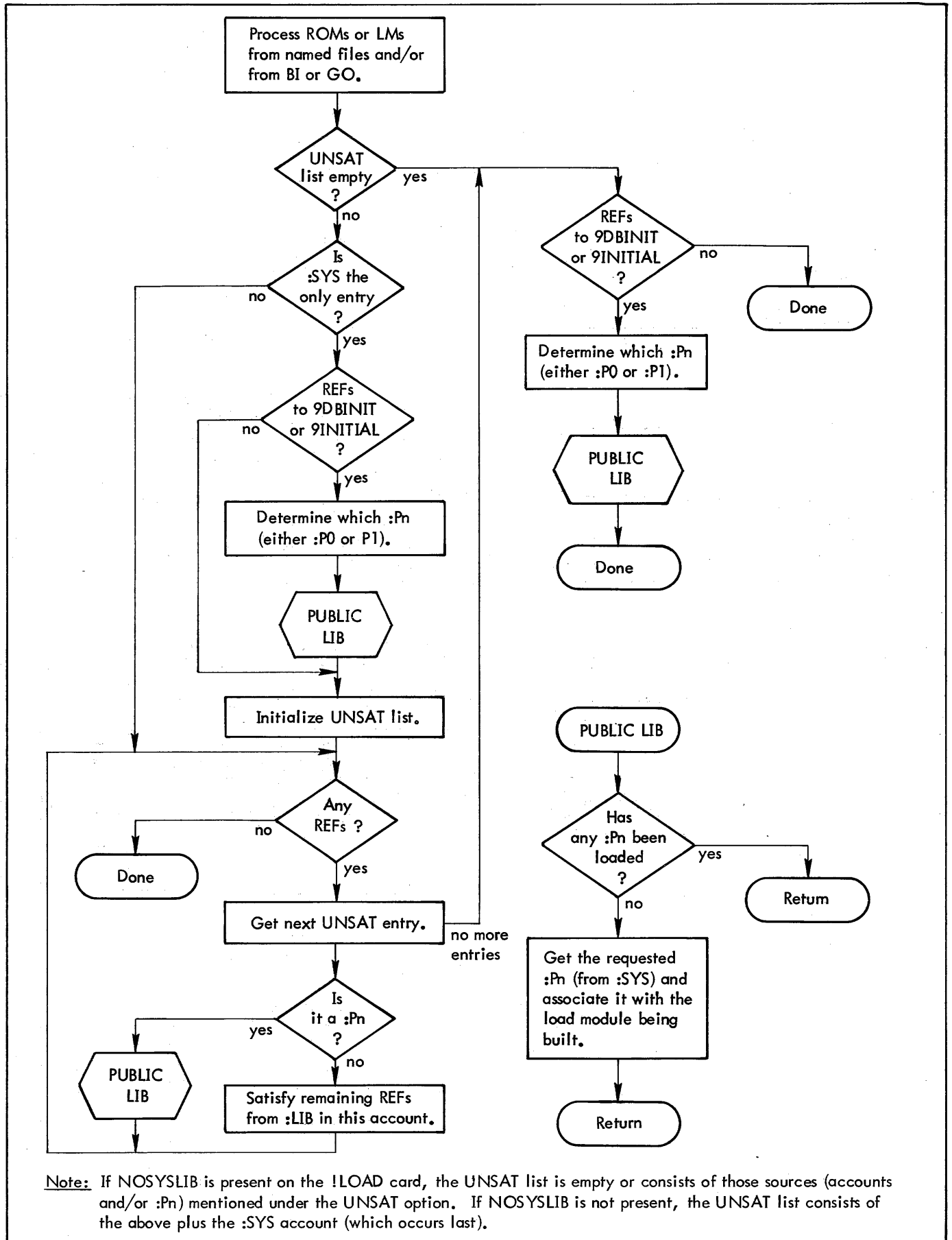
Figure 15. Generalized Library Load Process (Load)
