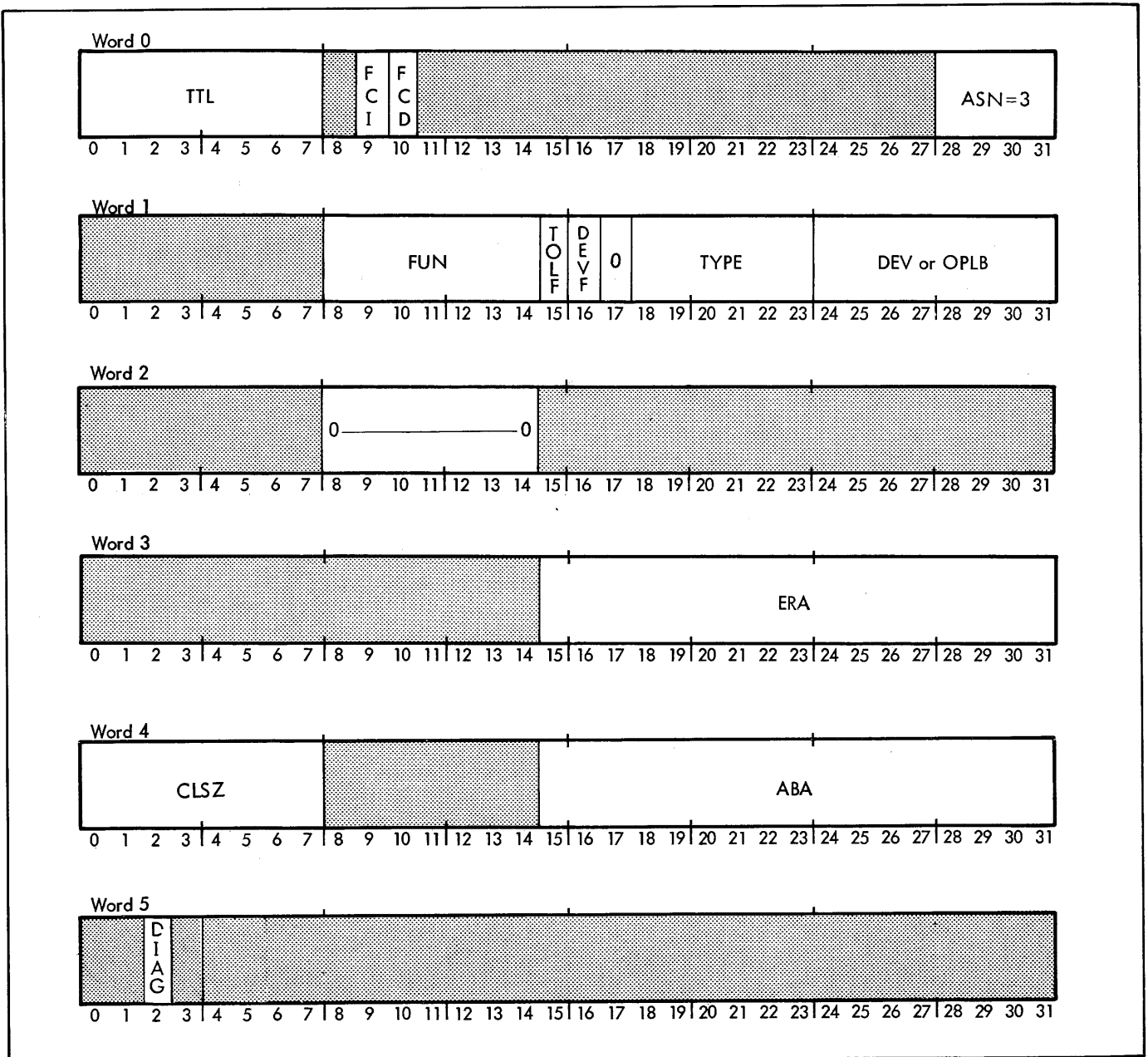
Figure 16. Format of the DDCB
