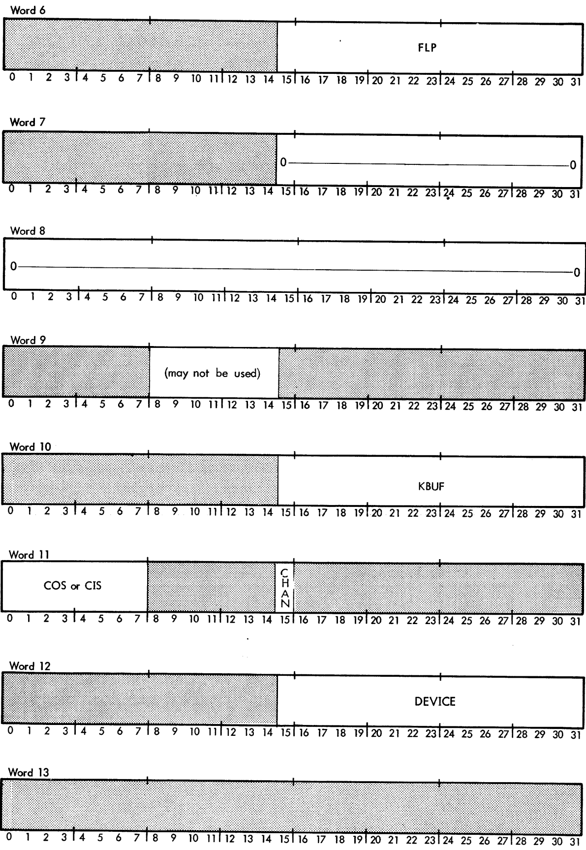
Figure 16. Format of the DDCB (cont.)
